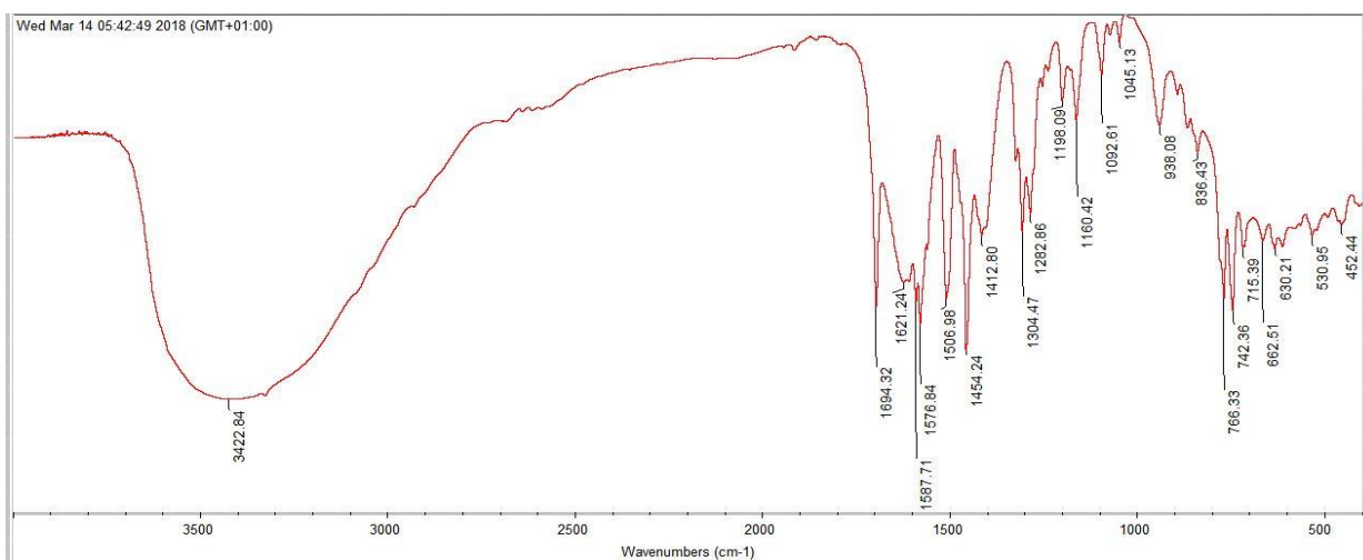
Figure 4: FTIR spectrum of \text{NiNaDCl}_2(\text{H}_2\text{O})_2
