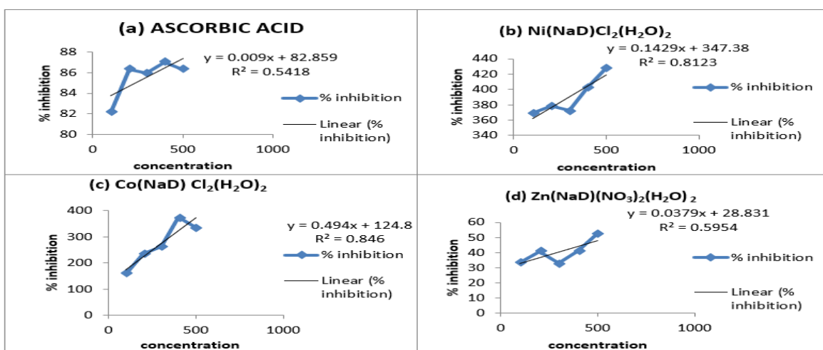
Figure 6: % inhibition versus concentration curve of (a) Ascorbic acid (b) Ni(NaD)Cl 2 (H 2 O) 2 (c) Co(NaD) Cl 2 (H 2 O) 2 (d) Zn(NaD)(NO 3 ) 2 (H 2 O) 2
