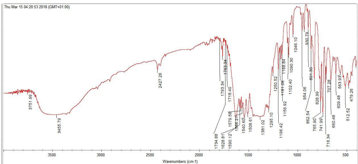
Figure 5: FTIR spectrum of \text{ZnNaD}(\text{NO}_3)_2(\text{H}_2\text{O})_2
