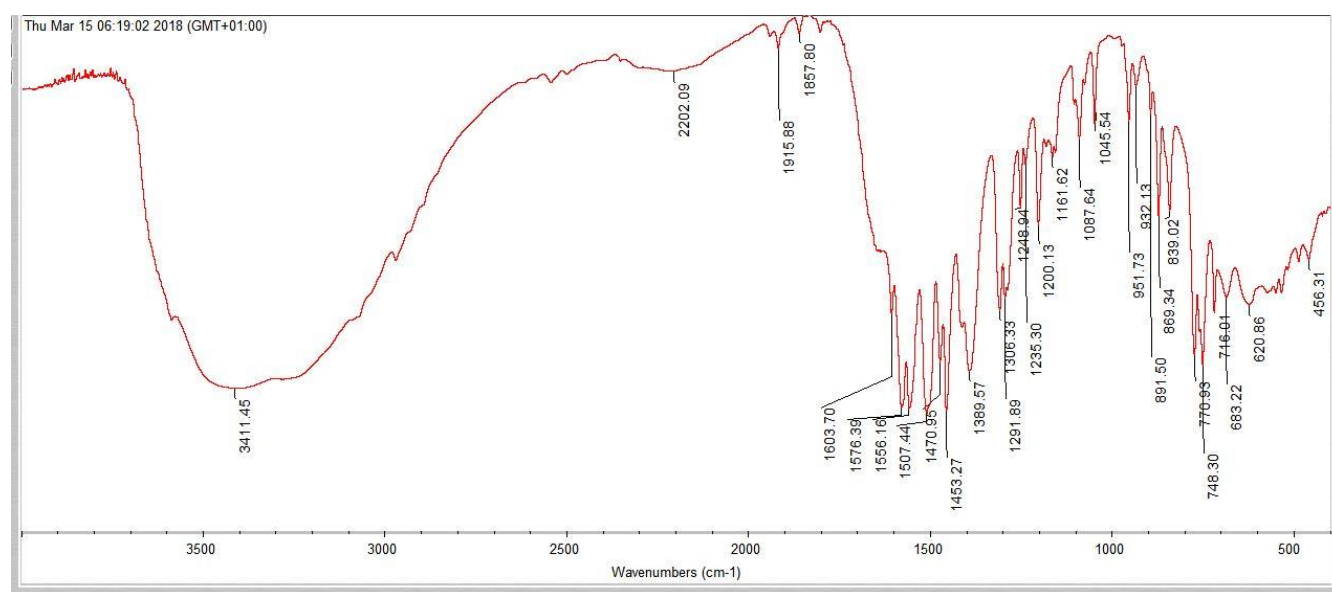
Figure 2: FTIR spectrum of sodium diclofenac (NaD)
