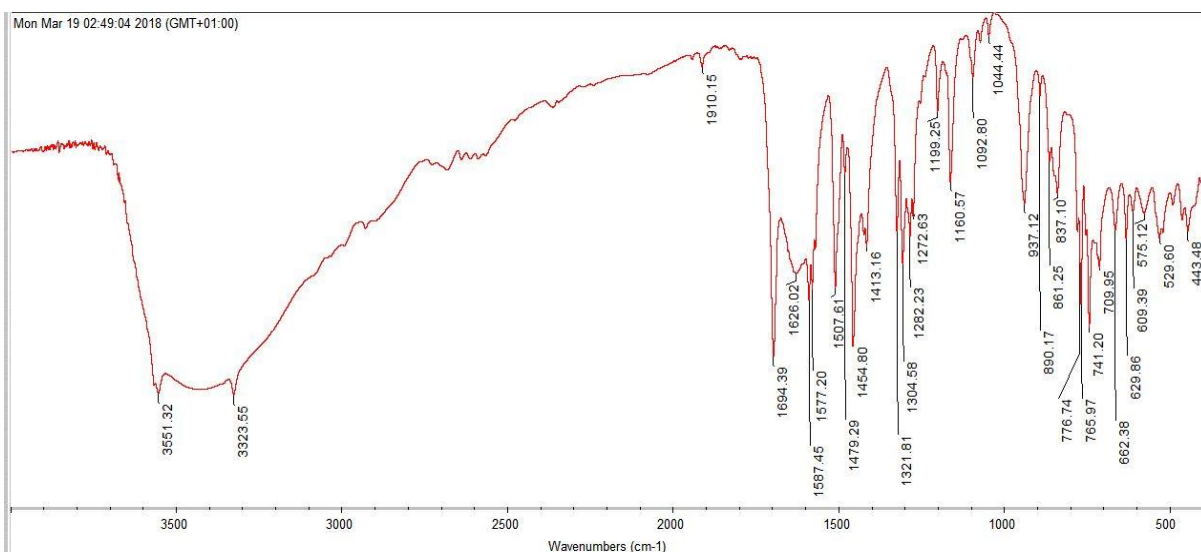
Figure 3: FTIR spectrum of \text{CoNaDCl}_2(\text{H}_2\text{O})_2
